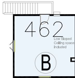
Pool House Upper Level
